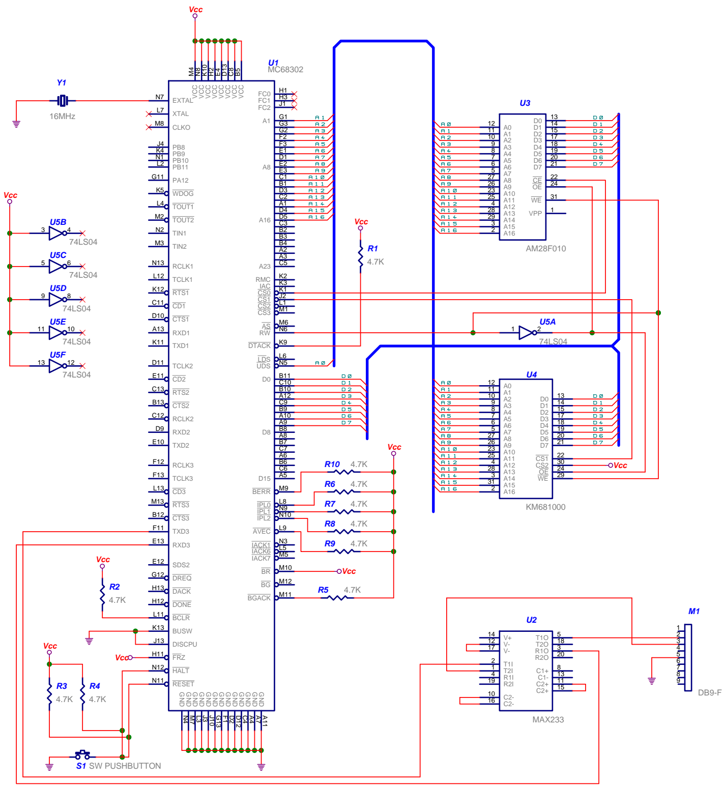
Tiny302 A minimal SBC based on MC68302 Jan 16, 2017, Rev 0.1 ©2017 H. Shen
