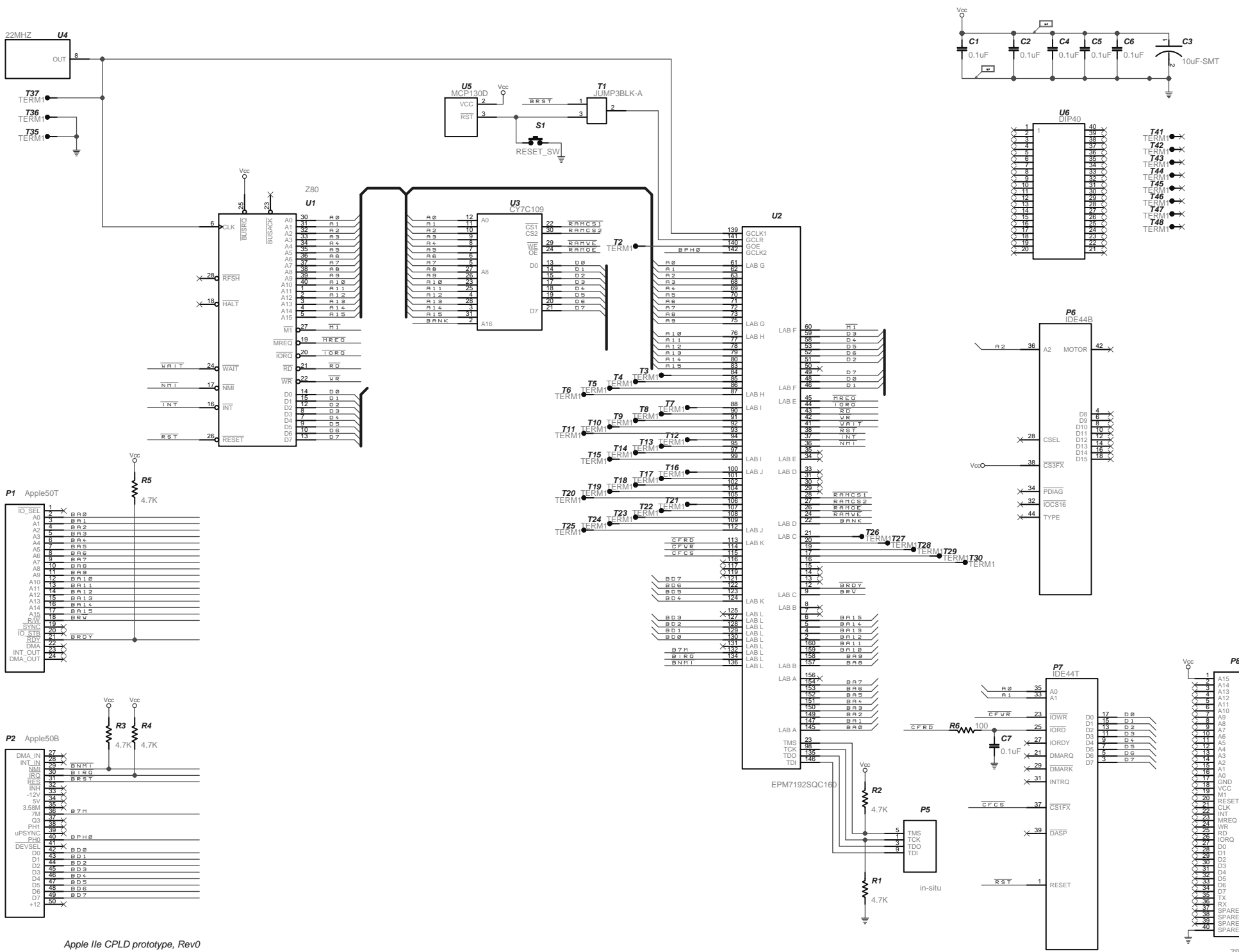
Apple IIe CPLD prototype, Rev0 12/22/21
