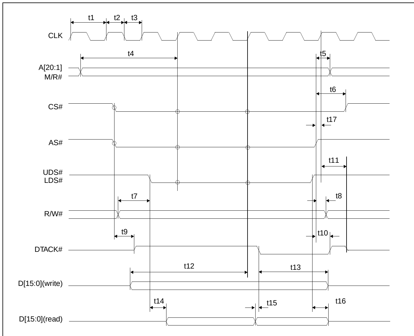
Figure 7-3: MC68000 Timing
